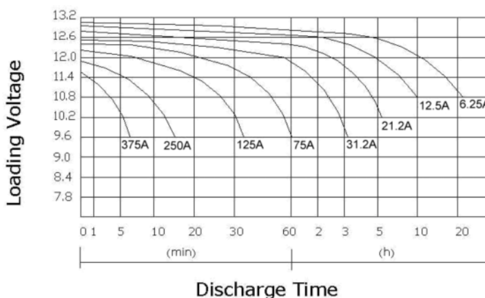
Discharge Characteristics(25°C/77 ° F)
