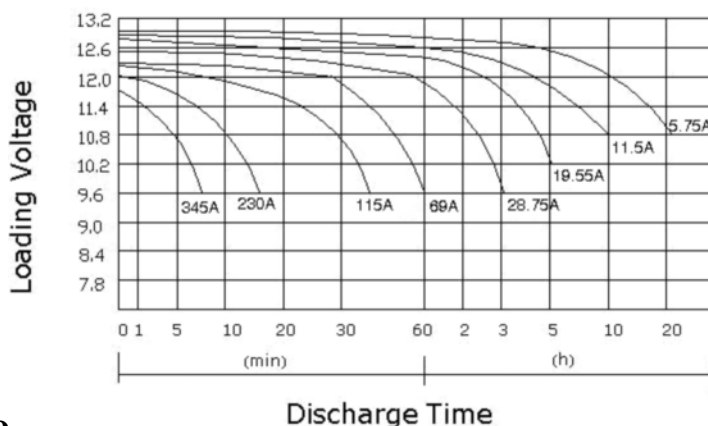
Discharge Characteristics(25°C/77 ° F)
